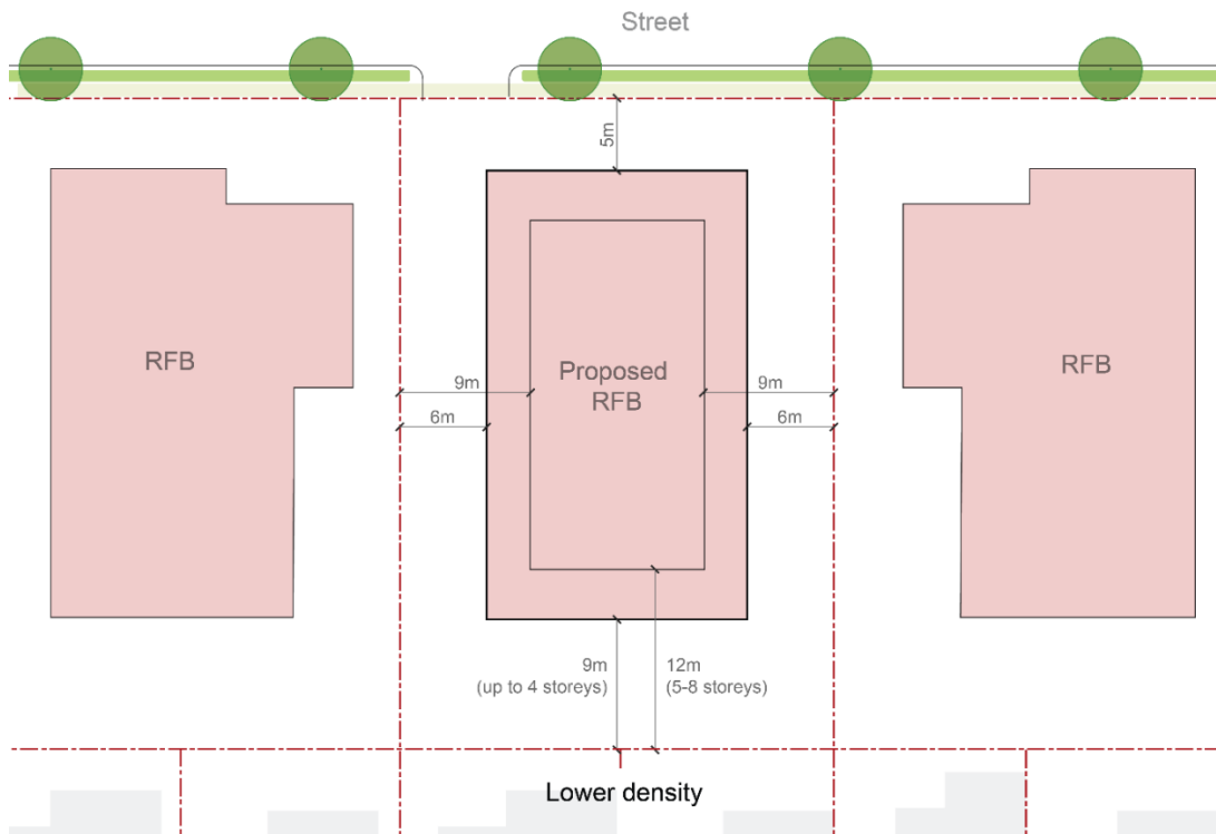
Figure 2: Application of the setbacks required for a residential flat building - with lower density interface (rear)
