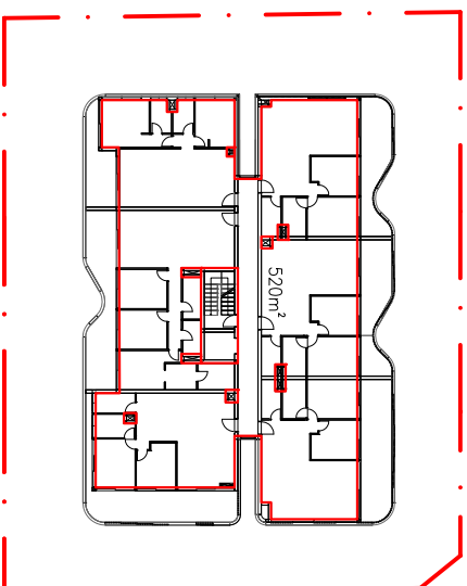
2. L1, L2 & L3 FLOOR PLAN FSR - 1:400
