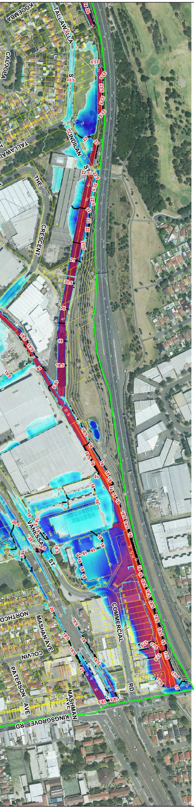
FIGURE : 1% AEP (100 year ARI) Depth and Flood Level - 150mm Cutoff - Map 2 of 23
