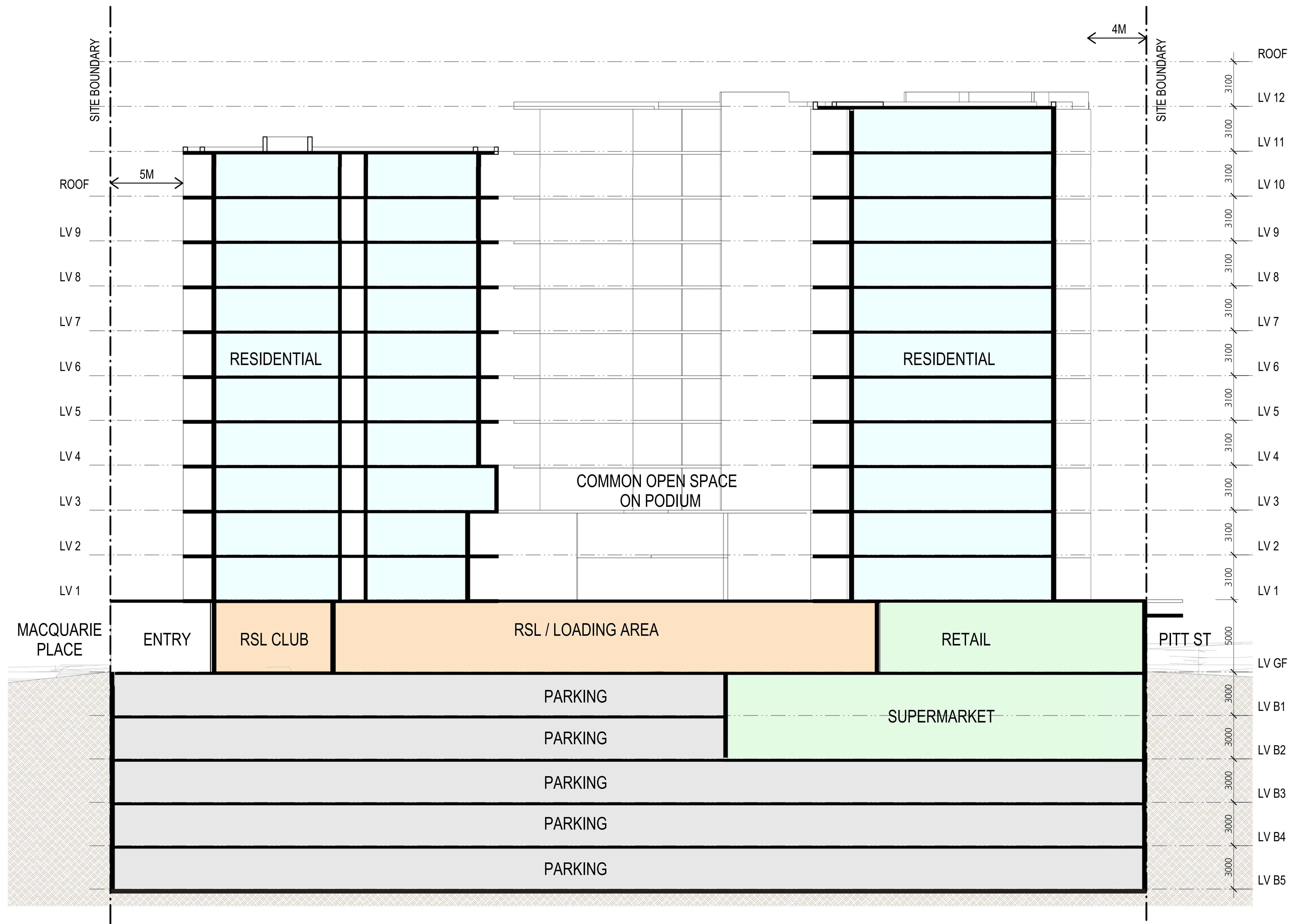
SCHEMATIC SECTION AA
